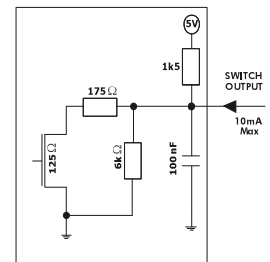
Equivalent circuit for the switch output
